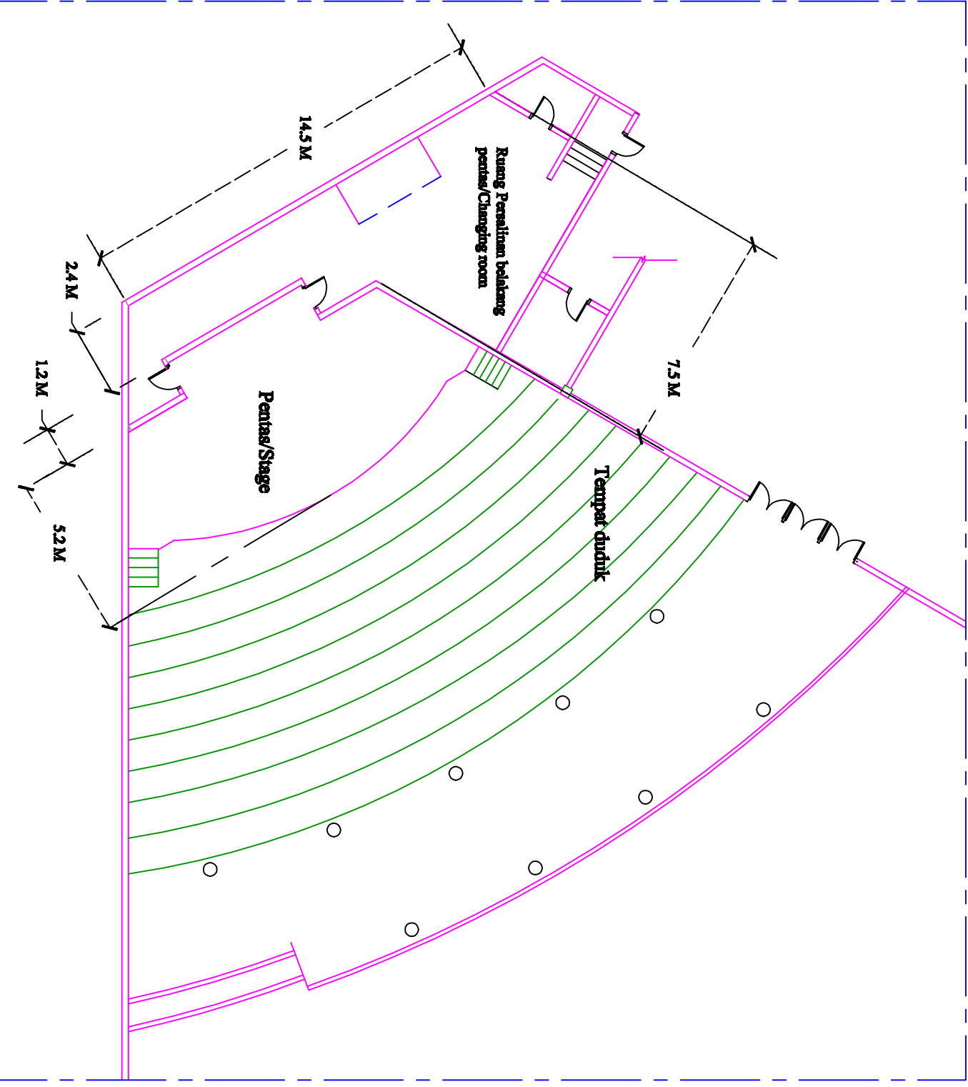
Plan lantai Pentas Terbuka/ Amphitheater layout plan
