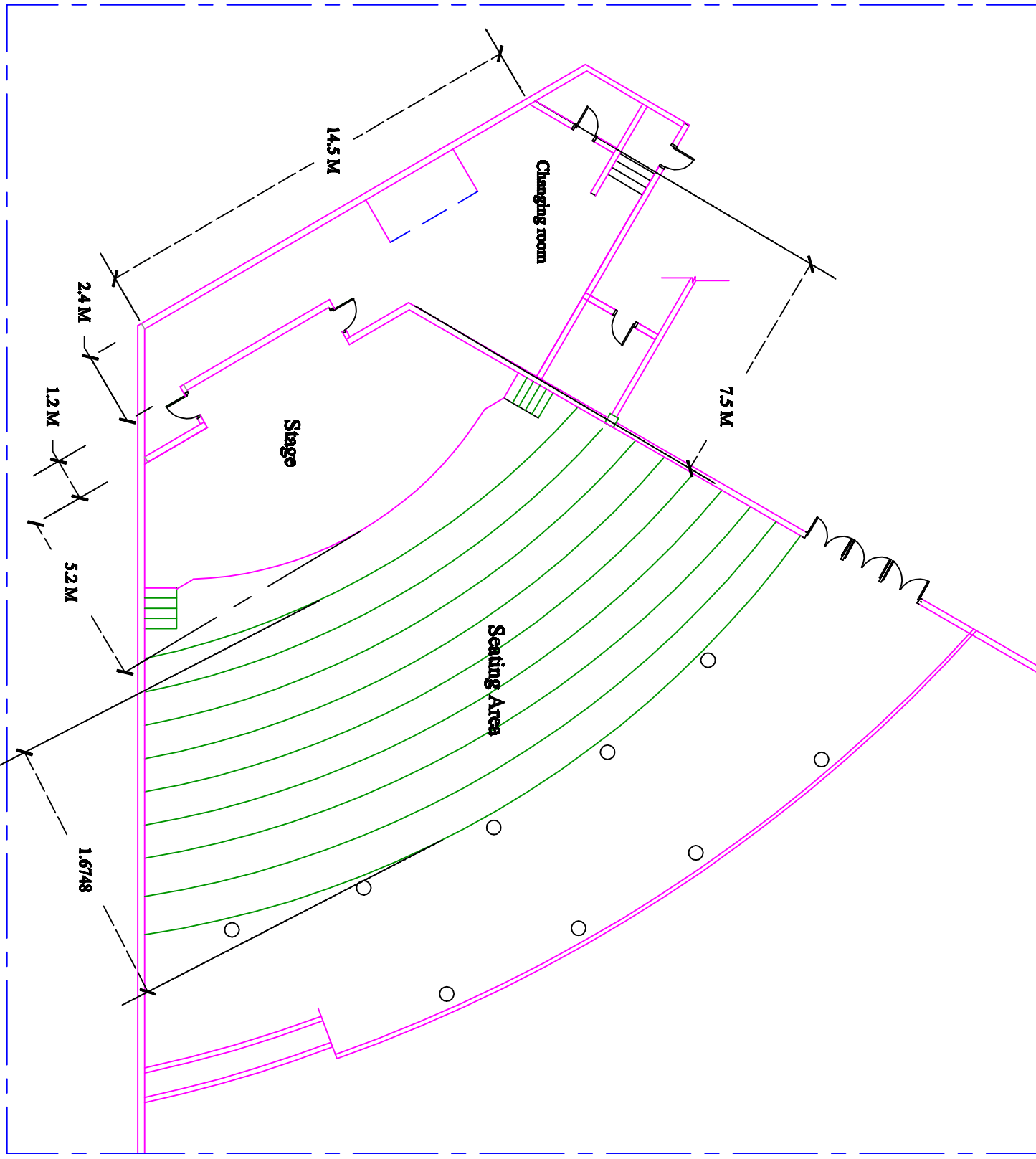
Amphitheatre layout plan
